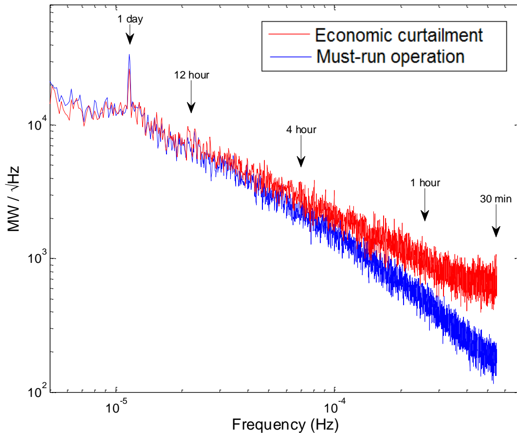
Figure 4.6: Power spectra of wind energy from one of the examined wind farms, under must-run (lower curve) and economic curtailment (upper curve) strategies. Increased variability under economic curtailment causes the power in higher frequencies to increase substantially: 350% at 30 minutes, 200% at 1 hour, and 35% at 4 hours.
