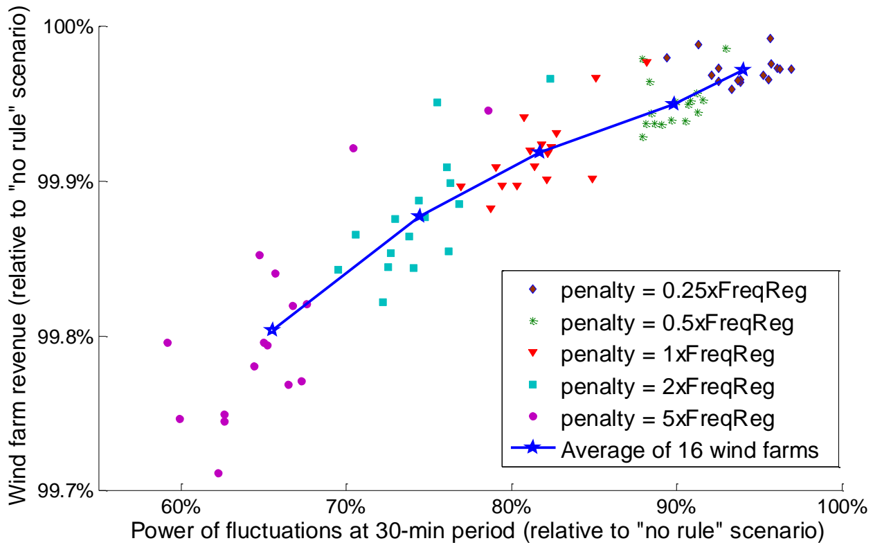
Figure 4.11: Change in revenue and 30-minute variability of sixteen wind farms under a market scenario with a limitation on both up- and down-ramping (ramp limit of 40% per 15-minute time step). The solid blue line and stars show the average results at each penalty level while the colored shapes show the results for individual wind farms.
