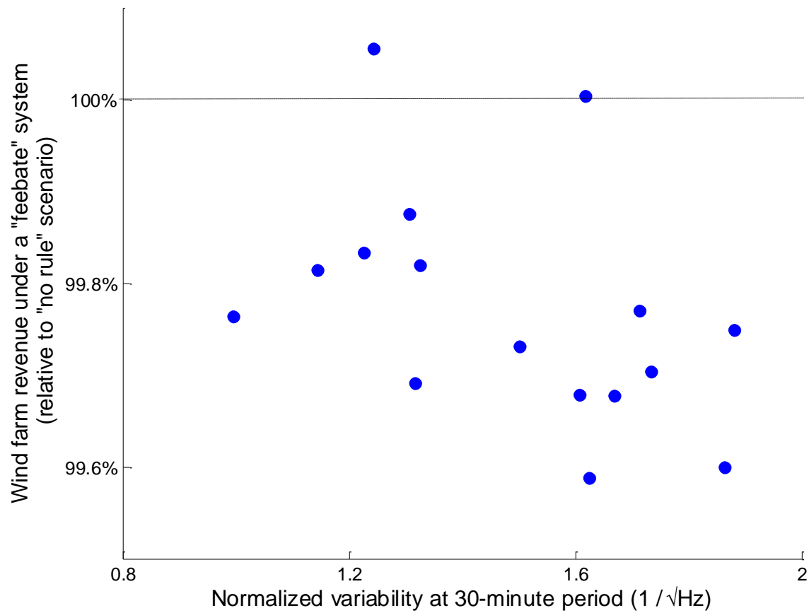
Figure 4.18: Wind farm revenue versus normalized natural variability at a period of 30-minutes for 16 wind farms in a market policy scenario where up- and down-ramping of wind is limited to 20% of nameplate capacity (per 15-minute step), penalties for over-ramping are five times the frequency regulation price, and all penalties are returned to wind generators in proportion to their installed capacity. The absolute variability at a period of 30-minutes (units of MW/√Hz) scales with the capacity of a wind farm and is normalized to installed capacity (units of MW/MW-√Hz , or 1/√Hz) in order to compare wind farms of different sizes. The x-axis shows the normalized variability of the actual measured wind data, showing the "natural" variability of that wind farm rather than their output under the ramp-limiting market policy. On average, wind farms lose revenue when over-ramping is penalized, even when all of the penalty payments are returned to wind. But a few wind farms acquire more revenue than they would if there were no limitation on wind ramping. The data show a slight downward trend, as wind farms with greater 30-minute variability lose more revenue.
