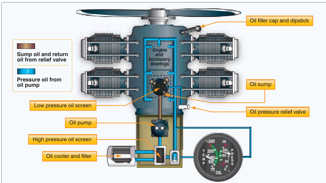
Figure 7-17. Wet-sump oil system.
