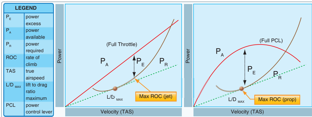
Figure 11-9. Comparison of maximum ROC between jet and propeller airplanes.
