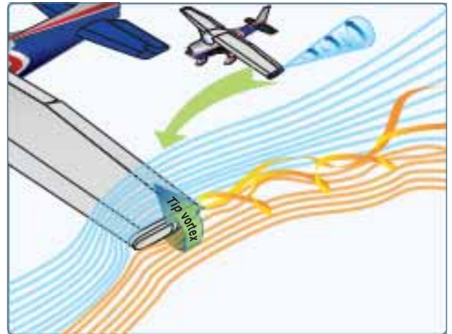
Figure 4-8. Tip vortex.
