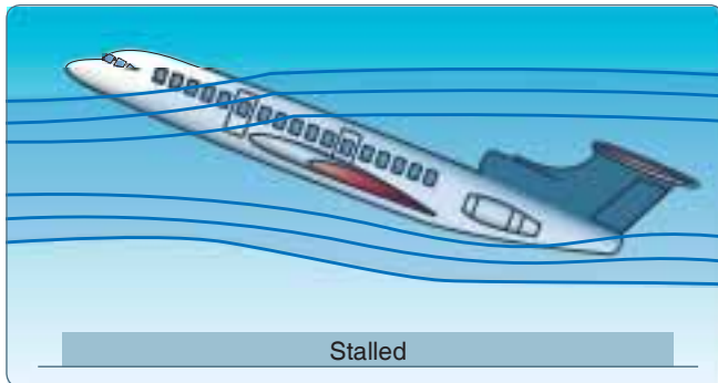
Figure 5-70. T-tail stall.
