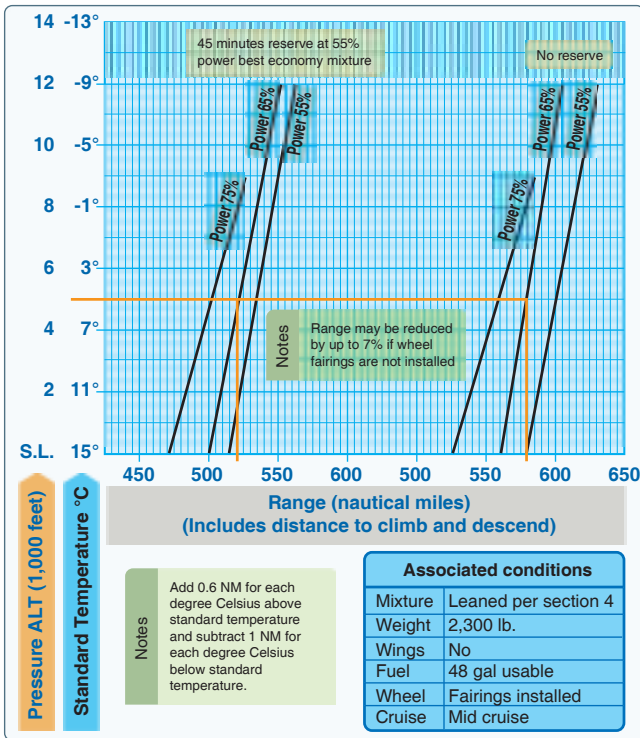
Figure 11-29. Best power mixture range.
