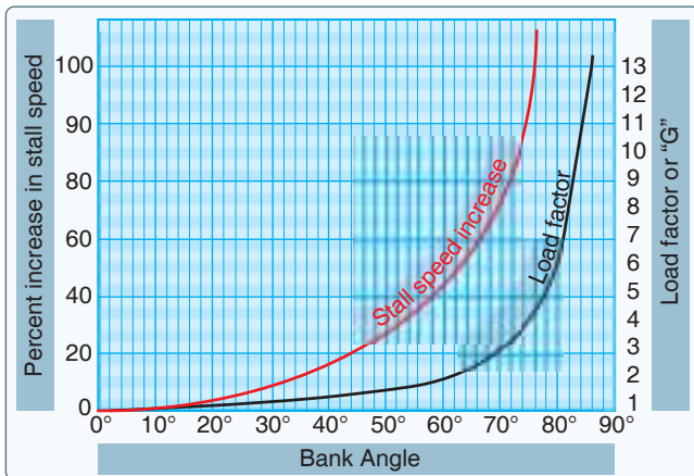
Figure 5-39. Increase in stall speed and load factor.
