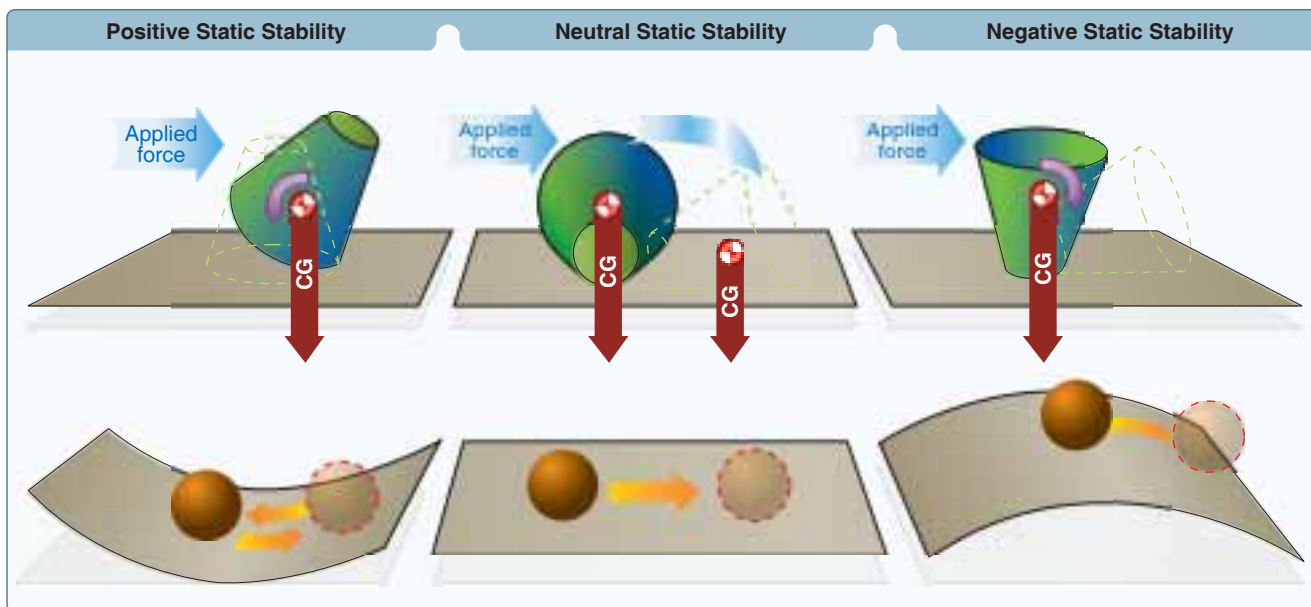
Figure 5-21. Types of static stability.
