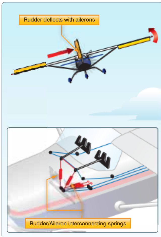
Figure 6-8. Coupled ailerons and rudder.
