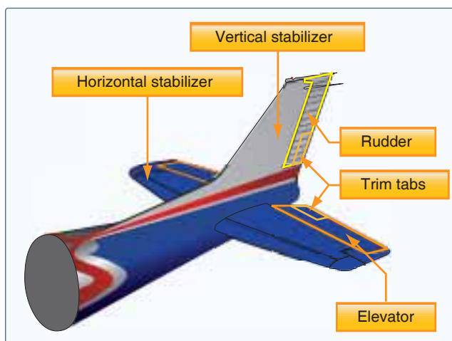
Figure 3-10. Empennage components.
