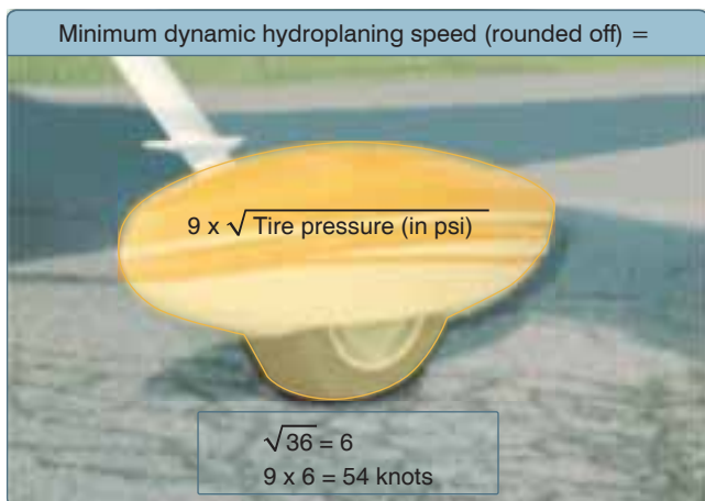
Figure 11-18. Tire pressure.
