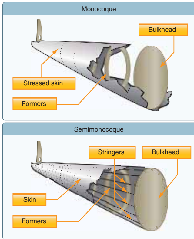
Figure 3-14. Semimonocoque and monocoque fuselage design.
