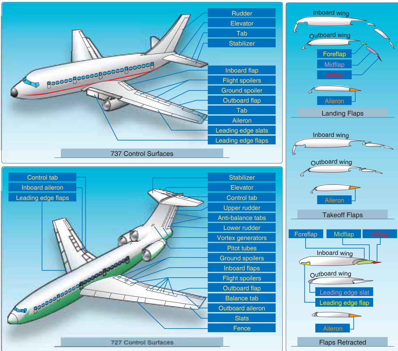
Figure 5-71. Control surfaces.
