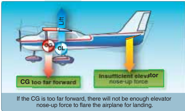
Figure 3-3. Center of gravity (CG).
