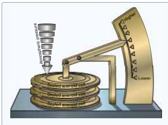
Figure 12-7. Aneroid barometer.
