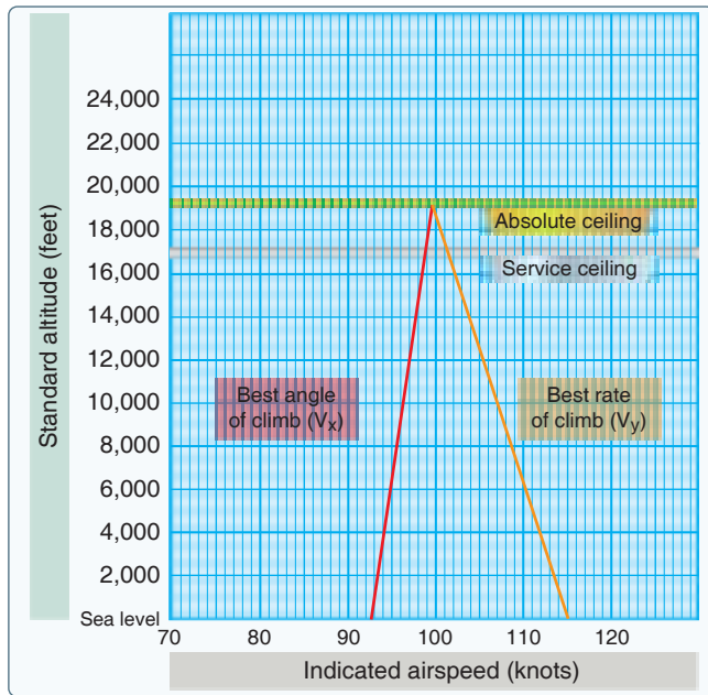
Figure 11-10. Absolute and service ceiling.
