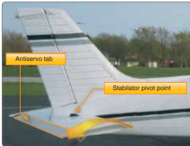
Figure 3-11. Stabilator components.
