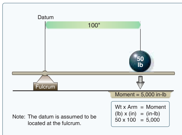
Figure 10-3. Determining moment.
