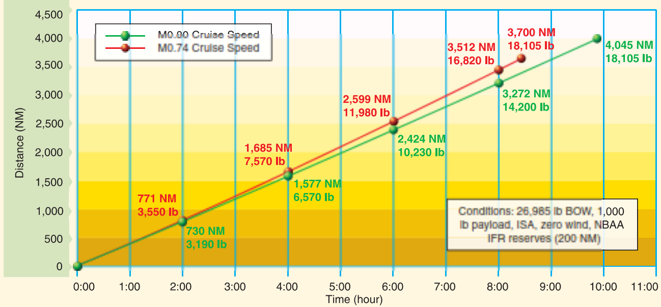
CHALLENGER 605 TIME AND FUEL VERSUS DISTANCE
