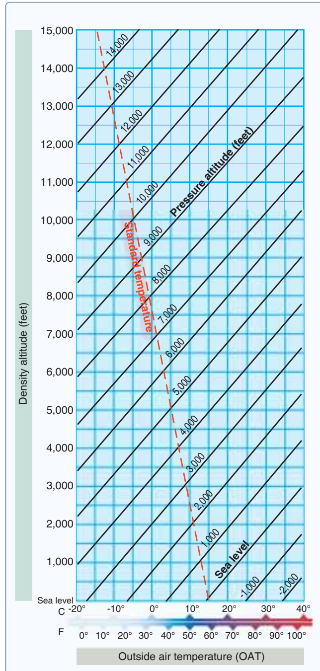
Figure 11-4. Density altitude chart.
