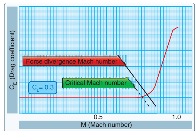
Figure 5-65. Critical Mach.
