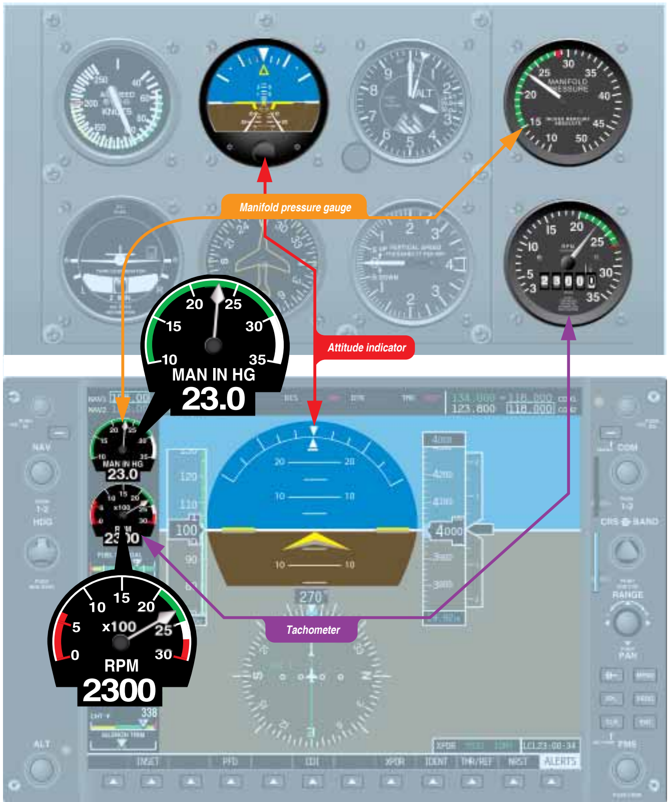
Figure 3-20. Control instruments.
