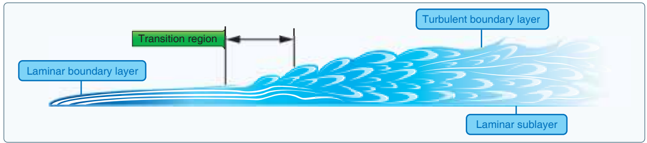
Figure 5-66. Boundary layer.
