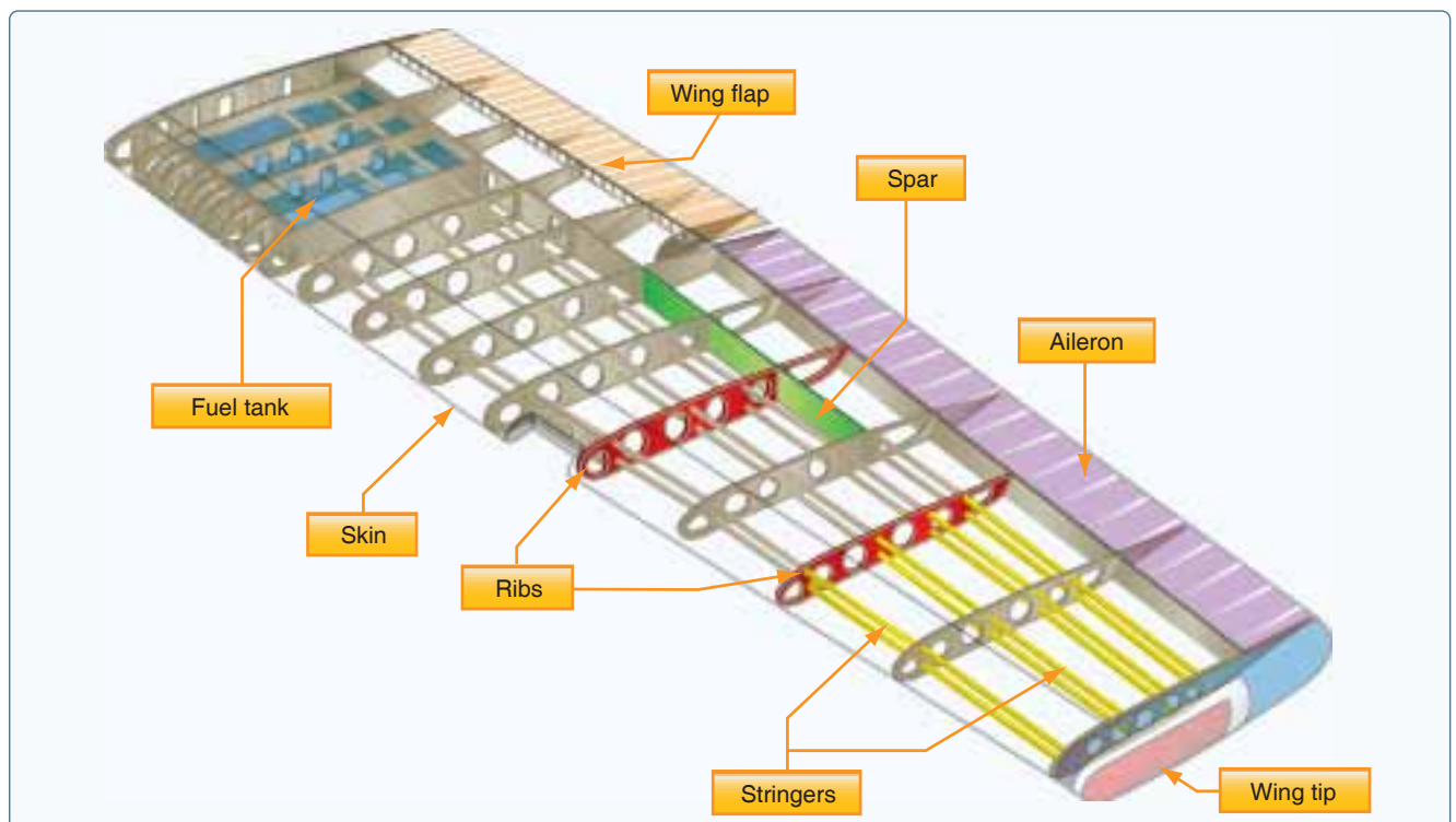
Figure 3-7. Wing components.
