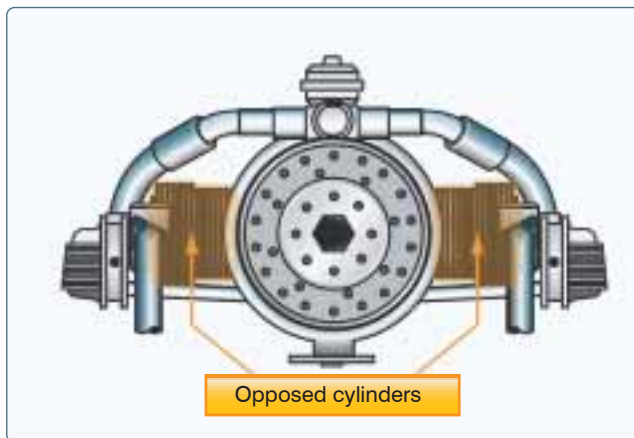
Figure 7-2. Horizontally opposed engine.
