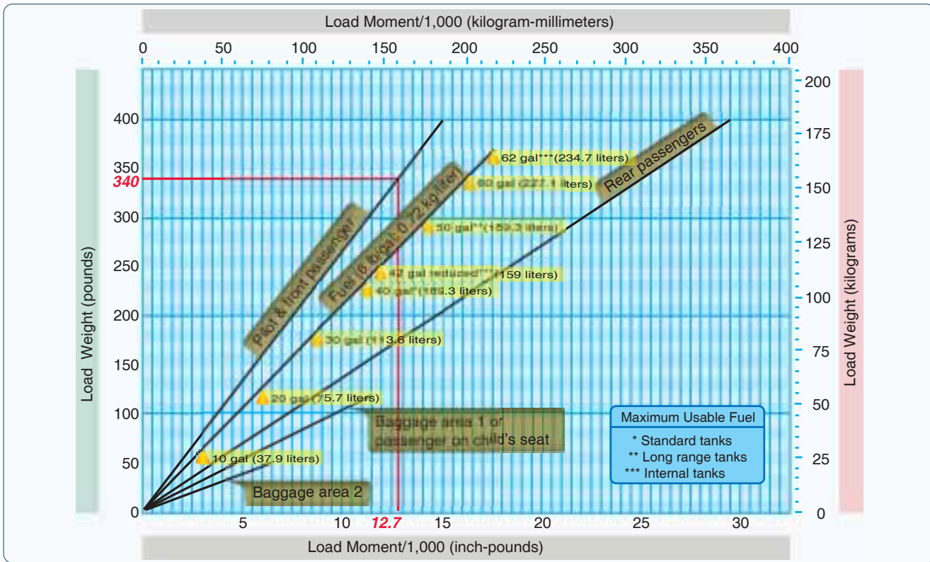
Figure 10-7. Loading graph.
