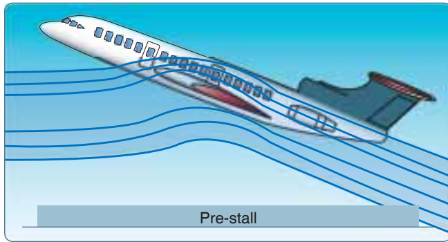
Figure 5-69. Wingtip pre-stall.
