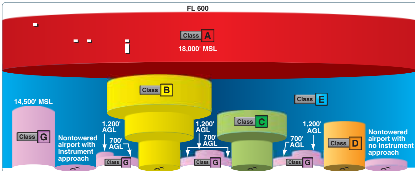
Figure 15-1. Airspace profile.
