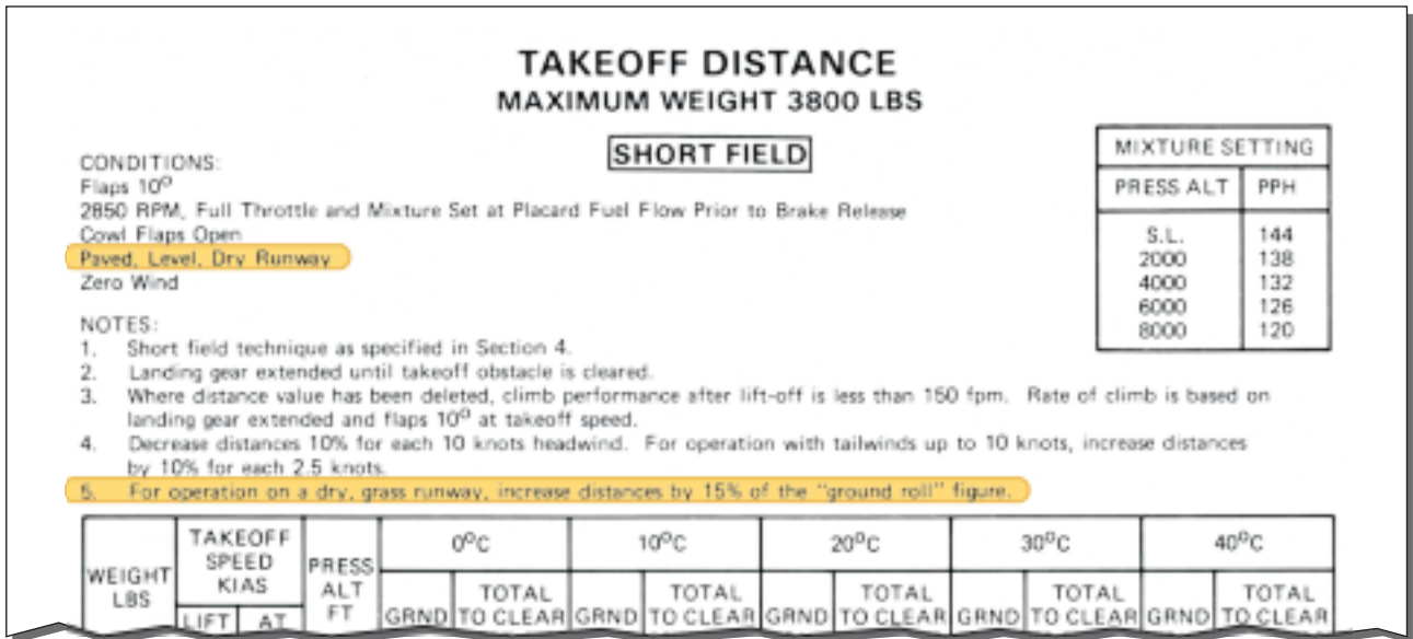
Figure 11-15. Takeoff distance chart.
