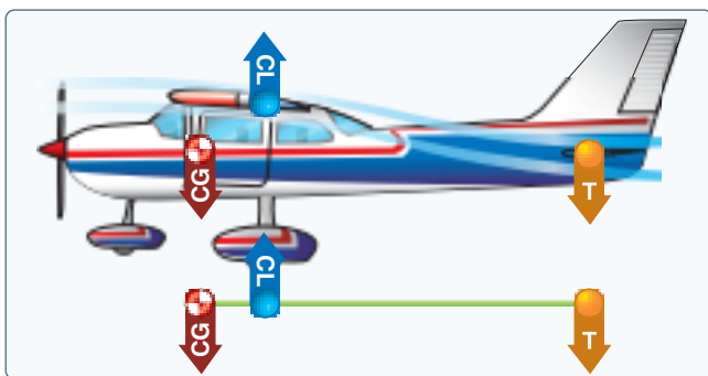
Figure 5-23. Longitudinal stability.
