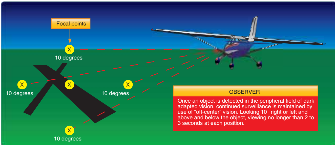
Figure 17-19. Off-center viewing.
