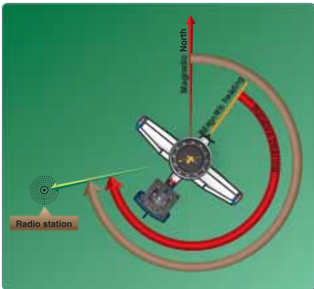
Figure 16-38. ADF terms.
