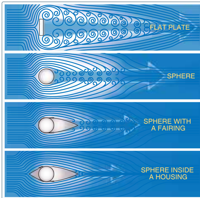
Figure 5-7. Form drag.
