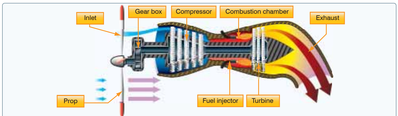
Figure 7-24. Turboprop engine.
