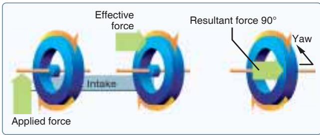
Figure 5-49. Gyroscopic precession.
