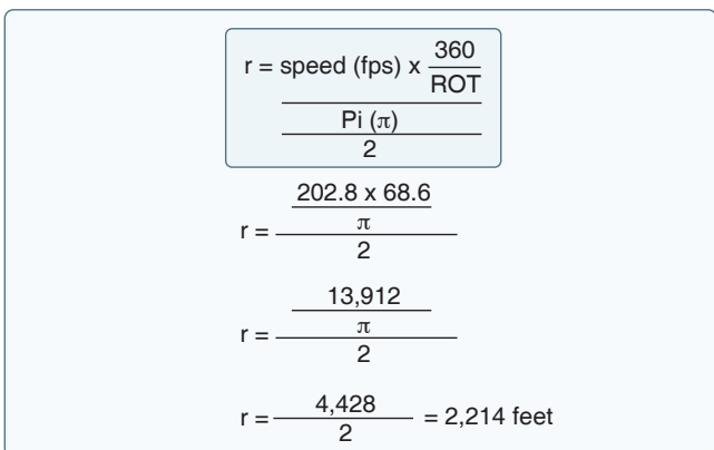
Figure 5-61. Another formula that can be used for radius.
