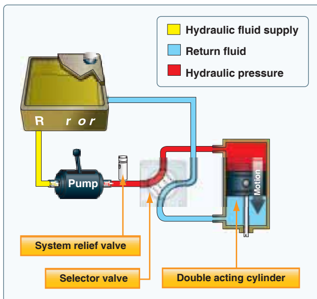
Figure 7-36. Basic hydraulic system.
