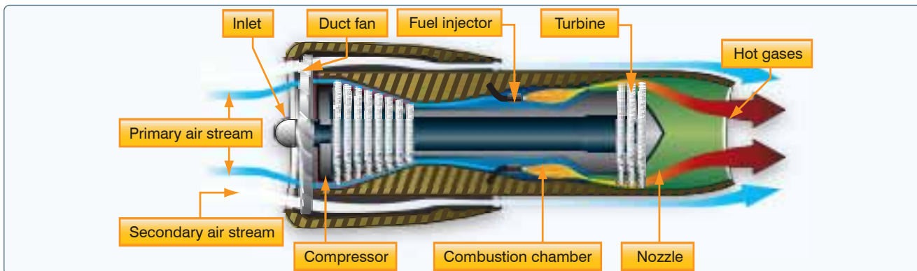
Figure 7-25. Turbofan engine.
