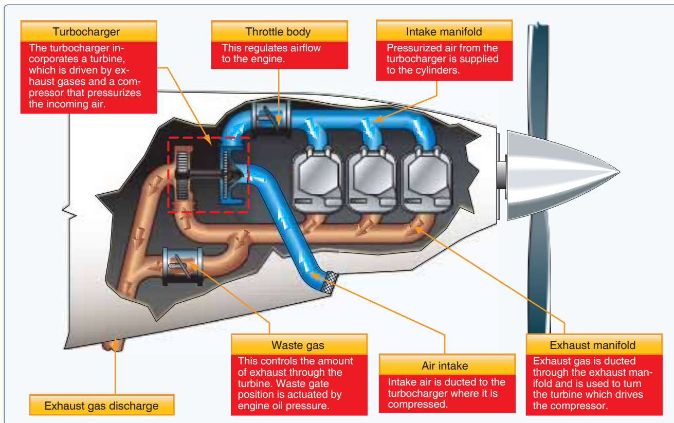
Figure 7-15. Turbocharger components.
