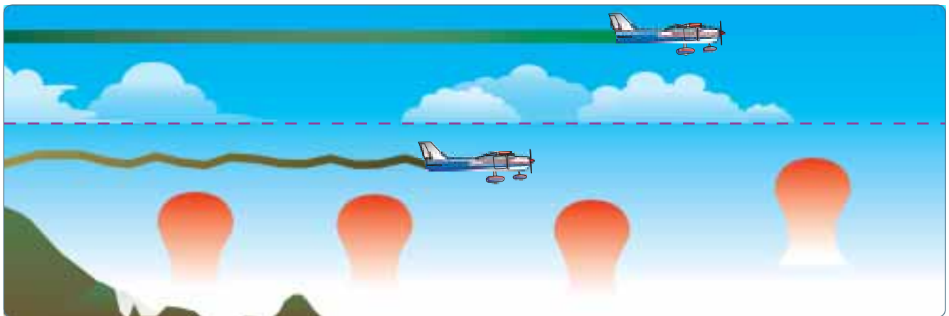
Figure 12-12. Convective turbulence avoidance.
