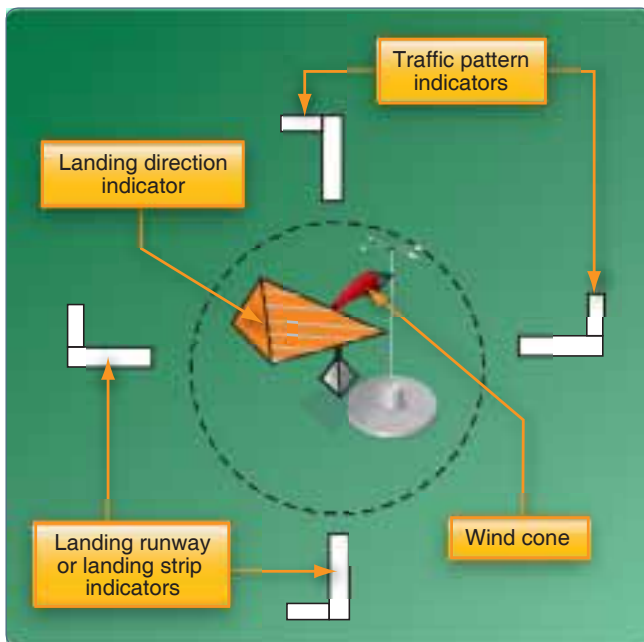
Figure 14-38. Segmented circle.
