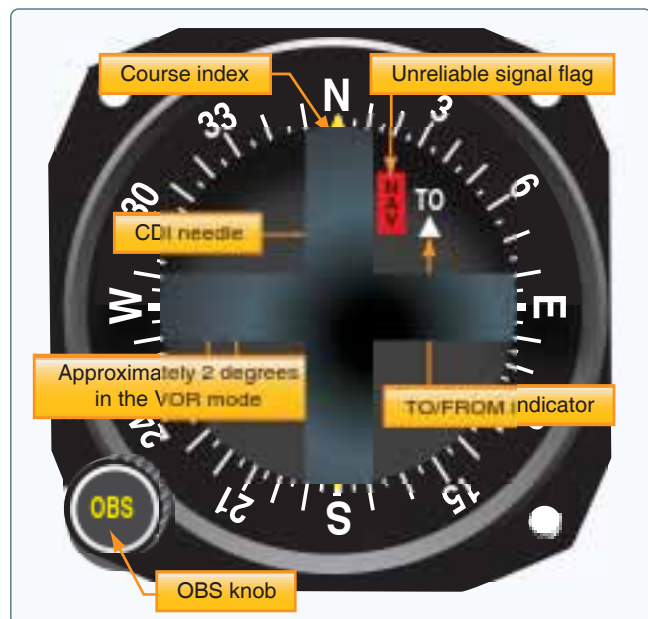
Figure 16-29. VOR indicator.
