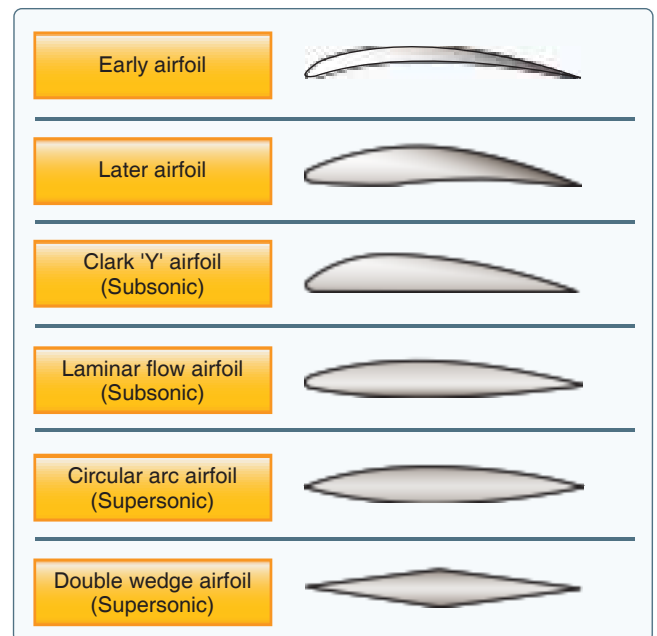
Figure 4-6. Airfoil designs.
