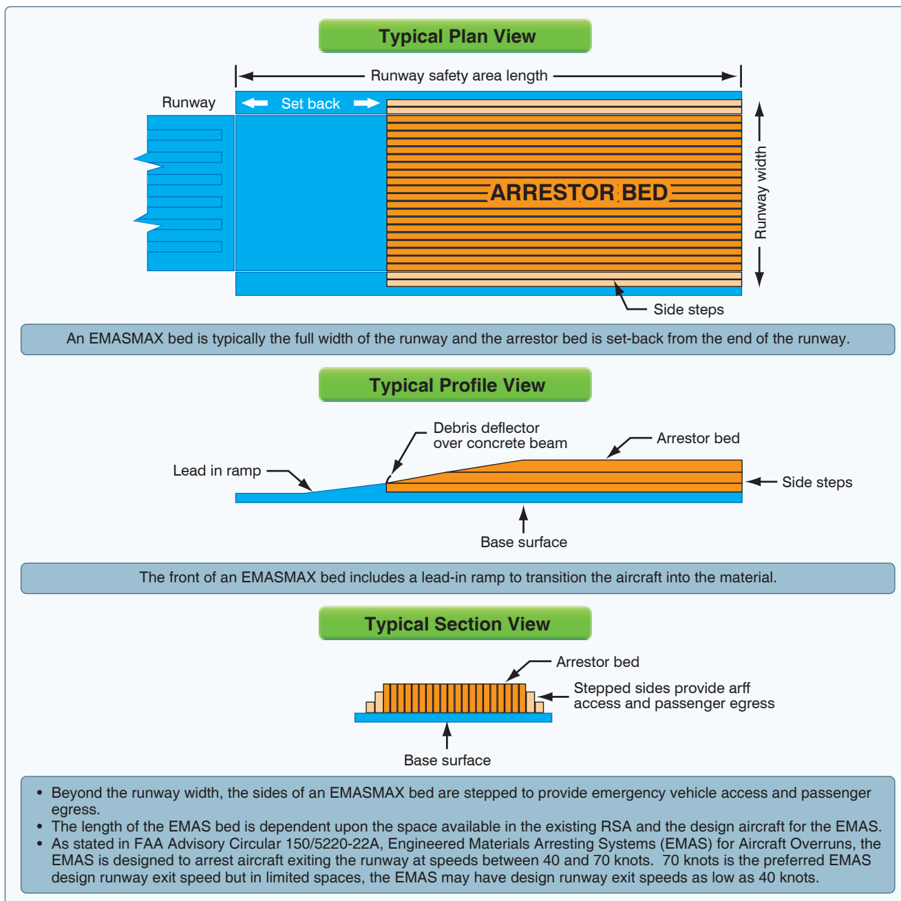
Figure 14-56. Diagram of an EMASMAX system.
