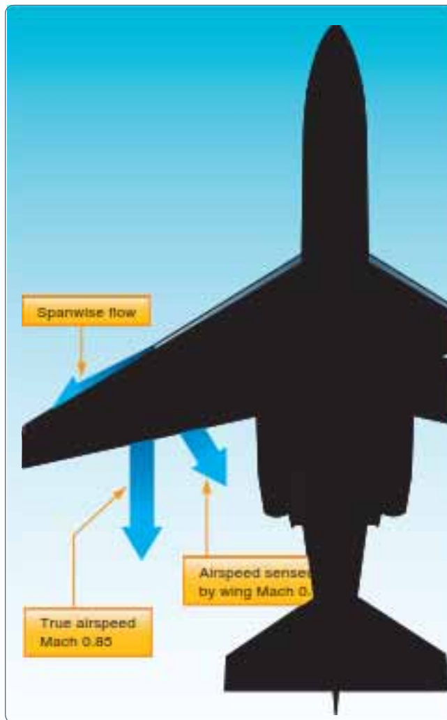
Figure 5-68. Sweepback effect.
