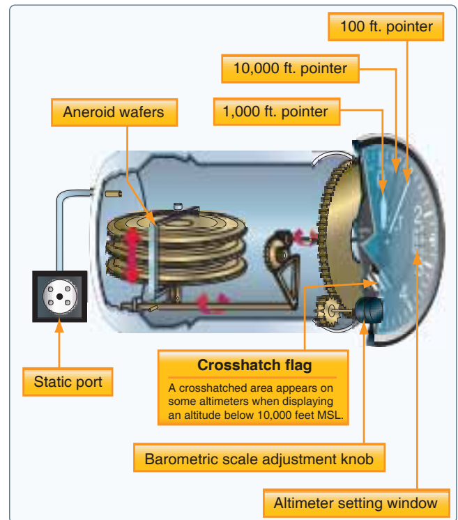
Figure 8-2. Altimeter.
