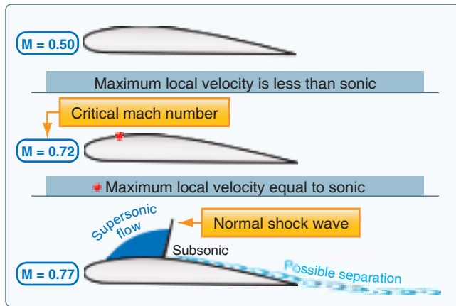
Figure 5-64. Wing airflow.
