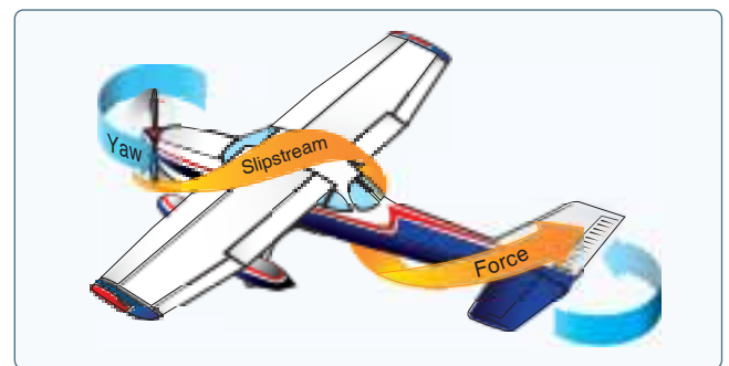
Figure 5-48. Corkscrewing slipstream.
