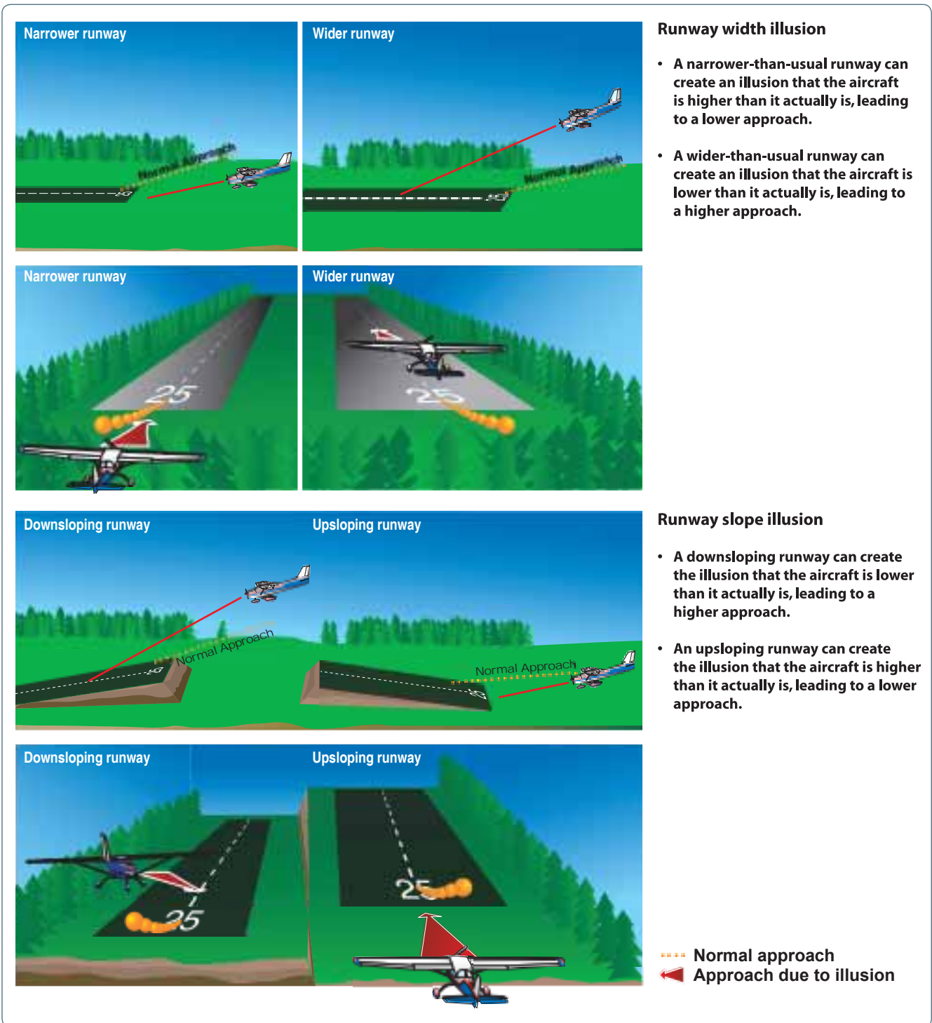
Figure 17-7. Runway illusions.
