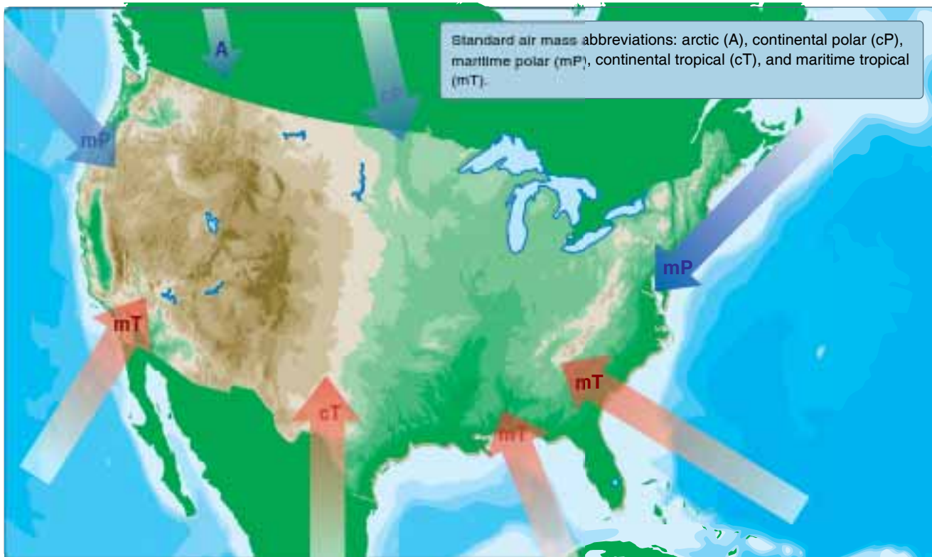
Figure 12-23. North American air mass source regions.
