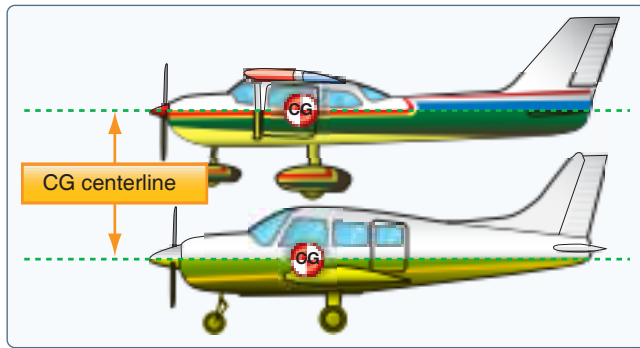
Figure 5-31. Keel area for lateral stability.
