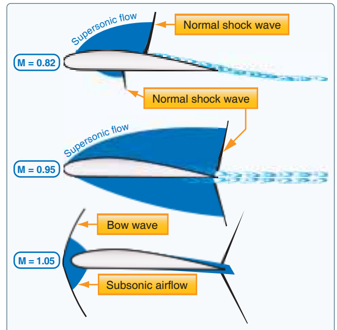
Figure 5-67. Shock waves.
