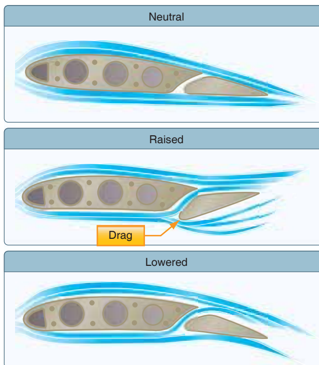
Figure 6-7. Frise-type ailerons.
