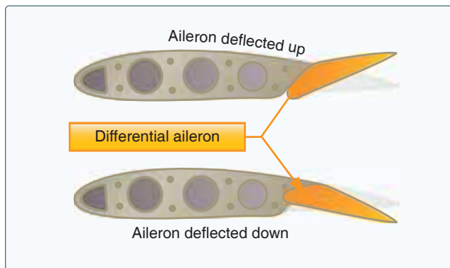
Figure 6-6. Differential ailerons.
