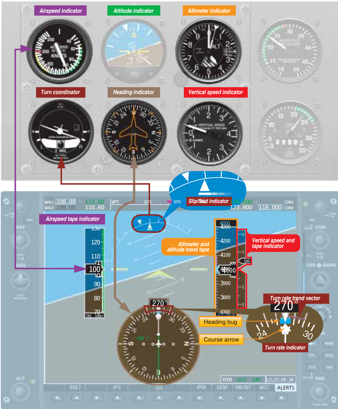
Figure 3-19. Performance instruments.
