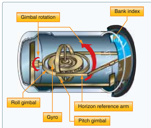
Figure 8-23. Attitude indicator.
