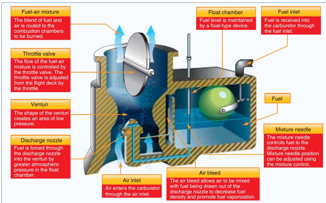
Figure 7-10. Float-type carburetor.
