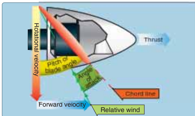
Figure 5-44. Propeller blade angle.
