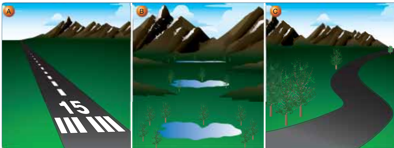
Figure 17-21. Geometric perspective.
