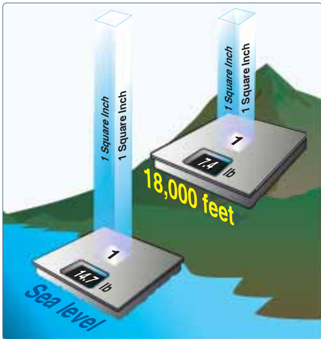
Figure 12-4. Atmosphere weights.
