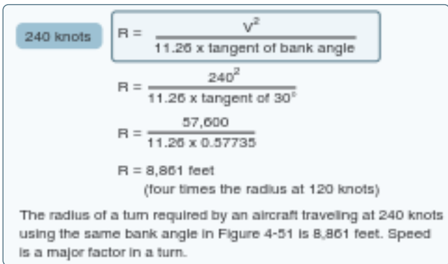
Figure 5-60. Radius at 240 knots.
