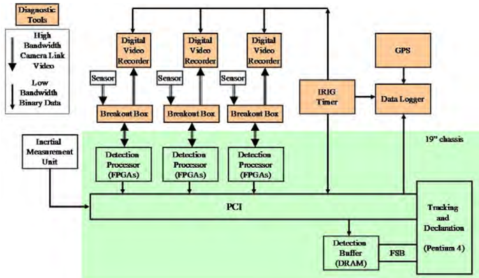
Figure D-9. The MITL SAA ATD Block Diagram
