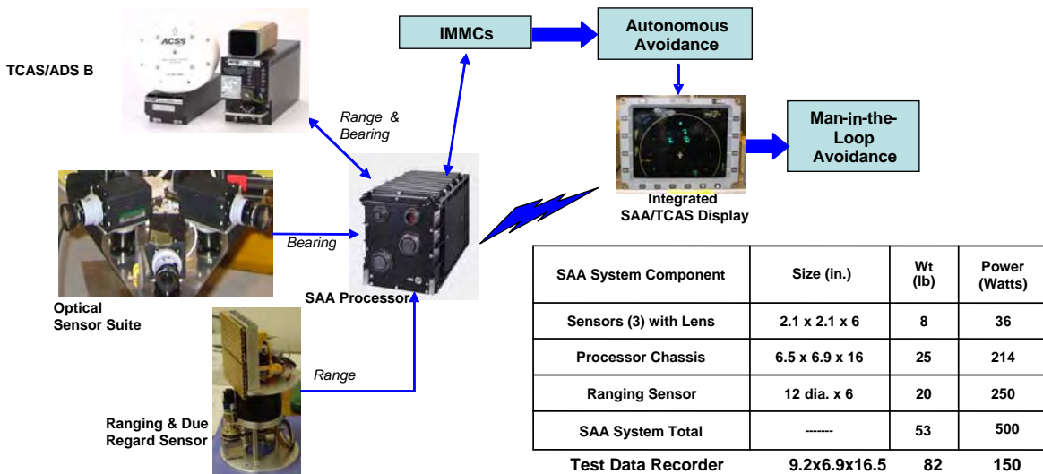
Figure D-16. Global Hawk Integrated SAA
