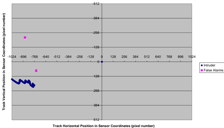
Figure D-8. False Alarm Analysis
