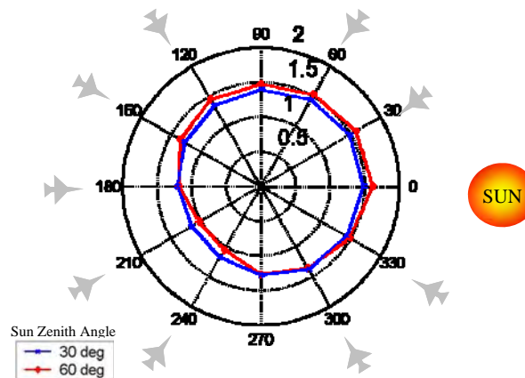
Figure D-2. OPEC Analysis Showing Human Detection Ranges in Nautical Miles
