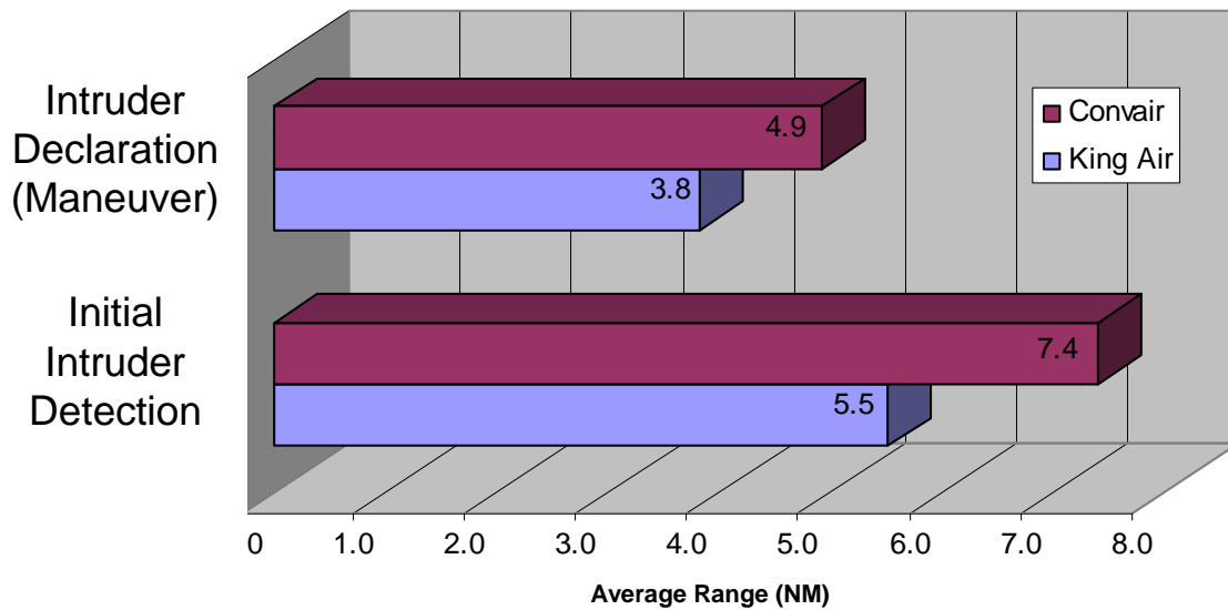
Figure D-13. Average Intruder Track and Declaration Ranges
