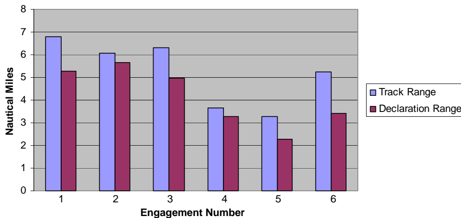
Figure D-7. ATDSS II Declaration Range Results
