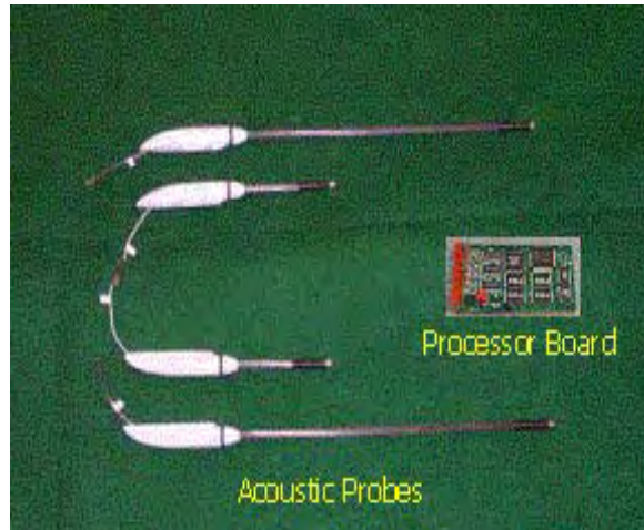
Figure 11. The Pancas Acoustic Sensor Probes and Signal Processor
