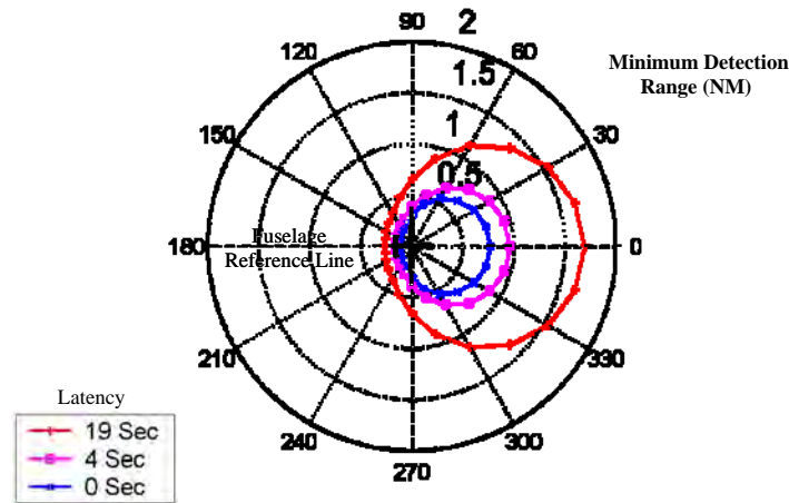
Figure D-3. Detection Range Requirements Software Example Results
